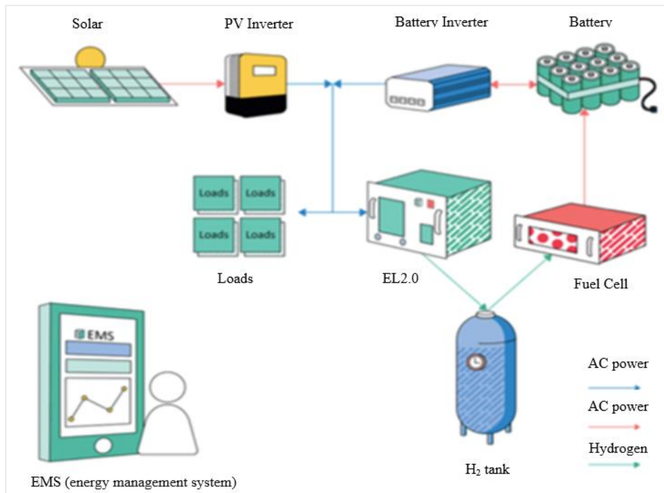
Figure 2: Component of waste-to-hydrogen (Wahh) microgrids
