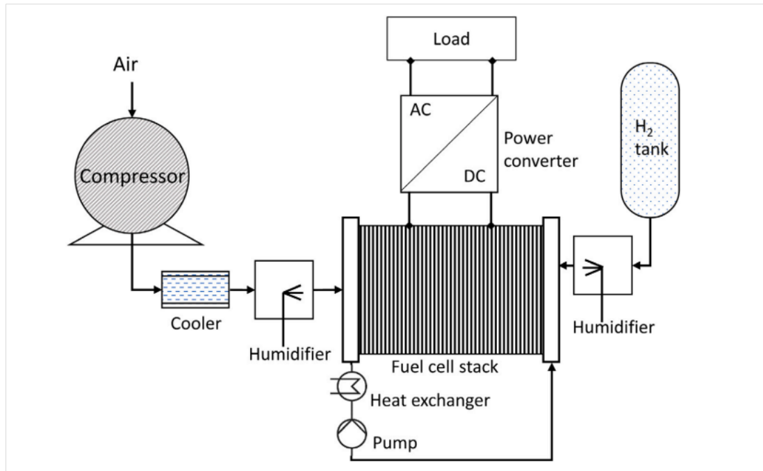
Figure 1: The configuration of a fuel cell system involves the pressurization and humidification of both hydrogen and air, which then pass through the fuel cell stack. The resulting electrical power generated is subsequently transmitted to a load through the utilization of an AC/DC power converter (Yue et al., 2021).
